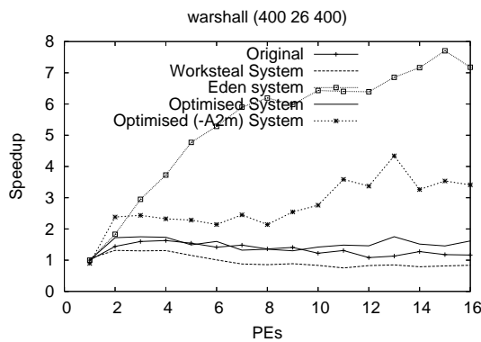
Speedups for shortest-paths-algorithm (400 nodes)
